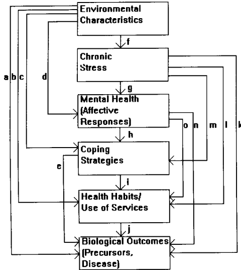
Figure 2 A range of models by which environmental characteristics may come to exert adverse biological outcomes on individuals. Segments b-o represent partial pathways that may concatenate to form more complex pathways.
